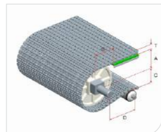
Type 型号: HS-1100B-N Pitch 节距: 15.2MM Thickness 厚度: 8.8MM Open area 开孔率: 28%
