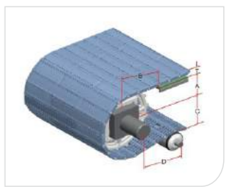
Type 型号: HS-502A-HD-D Pitch 节距: 25MM Thickness 厚度: 8.8MM Open area 开孔率: 0%
