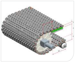
Type 型号: HS-500B Pitch 节距: 25MM Thickness 厚度: 11MM Open area 开孔率: 36%
