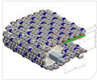
Type 型号: HS-300C Pitch 节距: 45MM Thickness 厚度: 19MM Open area 开孔率: 52%
