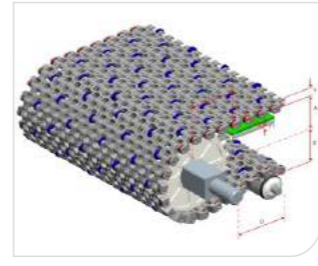
Type 型号: HS-501C Pitch 节距: 25MM Thickness 厚度: 14.5MM Open area 开孔率: 40%
