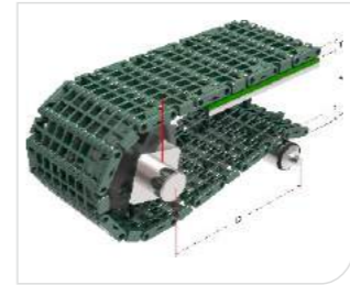
Type 型号: HS-F1000-84B-GB Pitch 节距: 25.4MM Thickness 厚度: 8.6MM Open area 开孔率: 42%
