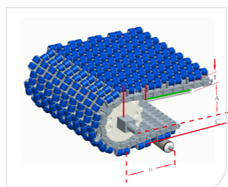
Type 型号: HS-1700C Pitch 节距: 37.5MM Thickness 厚度: 47.6MM Open area 开孔率: 26%
