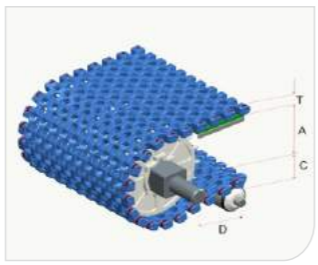
Type 型号: HS-500B-HD Pitch 节距: 25MM Thickness 厚度: 12.7MM Open area 开孔率: 36%
