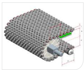
Type 型号: HS-501A Pitch 节距: 25MM Thickness 厚度: 13MM Open area 开孔率: 35%
