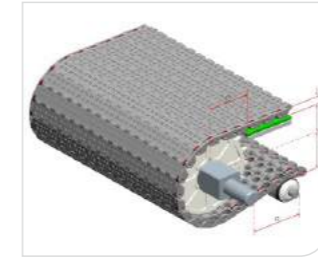
Type 型号: HS-502B Pitch 节距: 25MM Thickness 厚度: 13MM Open area 开孔率: 16%
