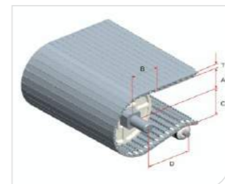
Type 型号: HS-1100A-N Pitch 节距: 15.2MM Thickness 厚度: 8.8MM Open area 开孔率: 0%
