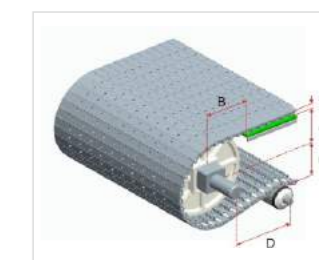
Type 型号: HS-1100AB-N Pitch 节距: 15.2MM Thickness 厚度: 8.8MM Open area 开孔率: 3%
