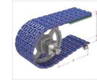
Type 型号: HS-3000B Pitch 节距: 25MM Thickness 厚度: 9.8MM Open area 开孔率: 25%
