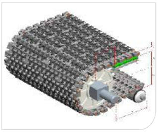
Type 型号: HS-500EL Pitch 节距: 25MM Thickness 厚度: 15.5MM Open area 开孔率: 36%
