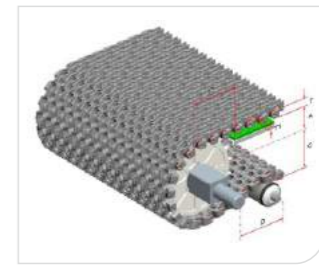
Type 型号: HS-600B Pitch 节距: 25MM Thickness 厚度: 18MM Open area 开孔率: 40%
