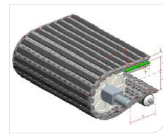
Type 型号: HS-502EL Pitch 节距: 25MM Thickness 厚度: 16MM Open area 开孔率: 0%
