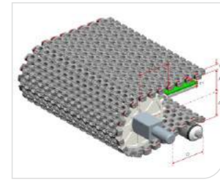
Type 型号: HS-501D Pitch 节距: 25MM Thickness 厚度: 15.5MM Open area 开孔率: 35%
