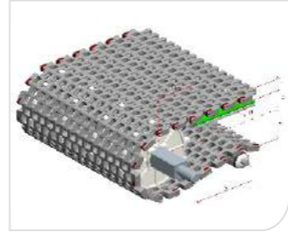
Type 型号: HS-300B-HD Pitch 节距: 45MM Thickness 厚度: 15MM Open area 开孔率: 38%
