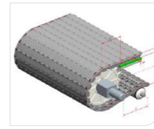
Type 型号: HS-502ZS Pitch 节距: 25MM Thickness 厚度: 14.2MM Open area 开孔率: 0%
