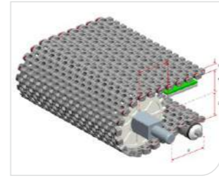
Type 型号: HS-501B Pitch 节距: 25MM Thickness 厚度: 13MM Open area 开孔率: 40%
