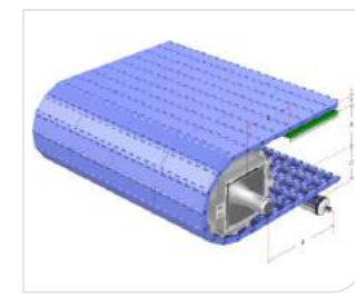
Type 型号: HS-502A-HD Pitch 节距: 25MM Thickness 厚度: 8.8MM Open area 开孔率: 0%
