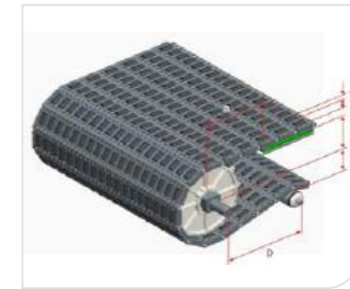
Type 型号: HS-3800-3C Pitch 节距: 50.8MM Thickness 厚度: 13MM Open area 开孔率: 3%
