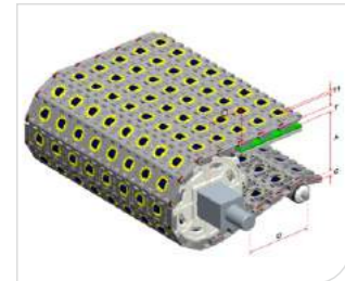
Type 型号: HS-800-2C Pitch 节距: 50.8MM Thickness 厚度: 18MM Open area 开孔率: 15%
