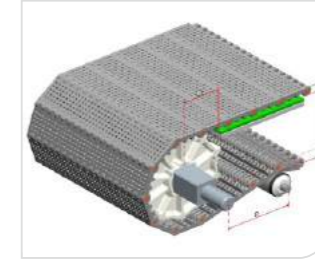
Type 型号: HS-101B Pitch 节距: 50.8MM Thickness 厚度: 16MM Open area 开孔率: 11.5%
