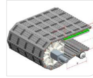
Type 型号: HS-100B-EL Pitch 节距: 50.8MM Thickness 厚度: 19.5MM Open area 开孔率: 18%
