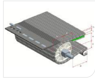
Type 型号: HS-700D-N Pitch 节距: 27.2MM Thickness 厚度: 14.4MM Open area 开孔率: 38%
