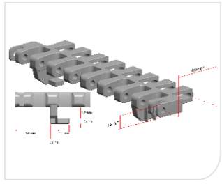
Type 型号: HS-300B-HD-GB Pitch 节距: 45MM Thickness 厚度: 15MM Open area 开孔率: 38%
