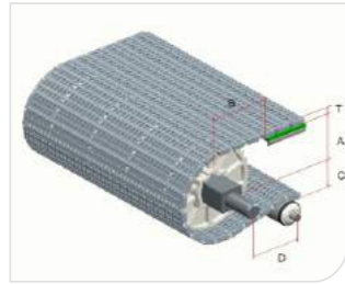
Type 型号: HS-700B-N Pitch 节距: 27.2MM Thickness 厚度: 8.8MM Open area 开孔率: 38%
